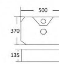
OVS-A464 Size:500x370x135mm
