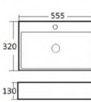
OVS-A394 Size:555x320x130mm
